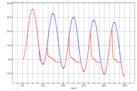
Figure 6: Transient simulation of a 3000 A / 1 A, 5P20, 30 VA CT with R_{CT} < 10 \Omega
