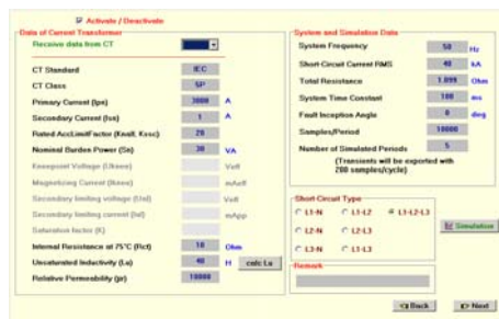
Fig. 5: Transient simulation window
