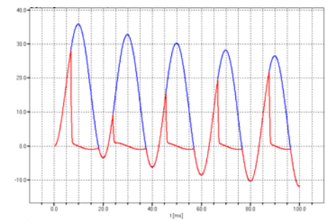
Figure 7: Transient simulation of the optimized 3000 A / 1 A, 5P20, 2.5 VA CT with R_{CT} < 5 \Omega
